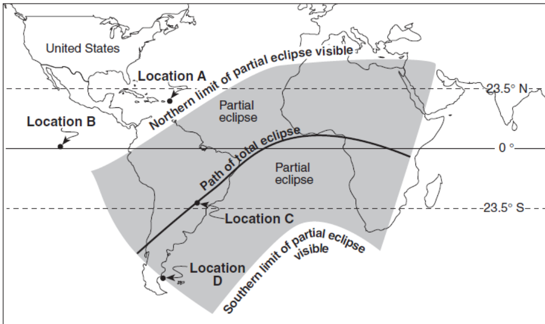
Solar Eclipse May 20, 1947
