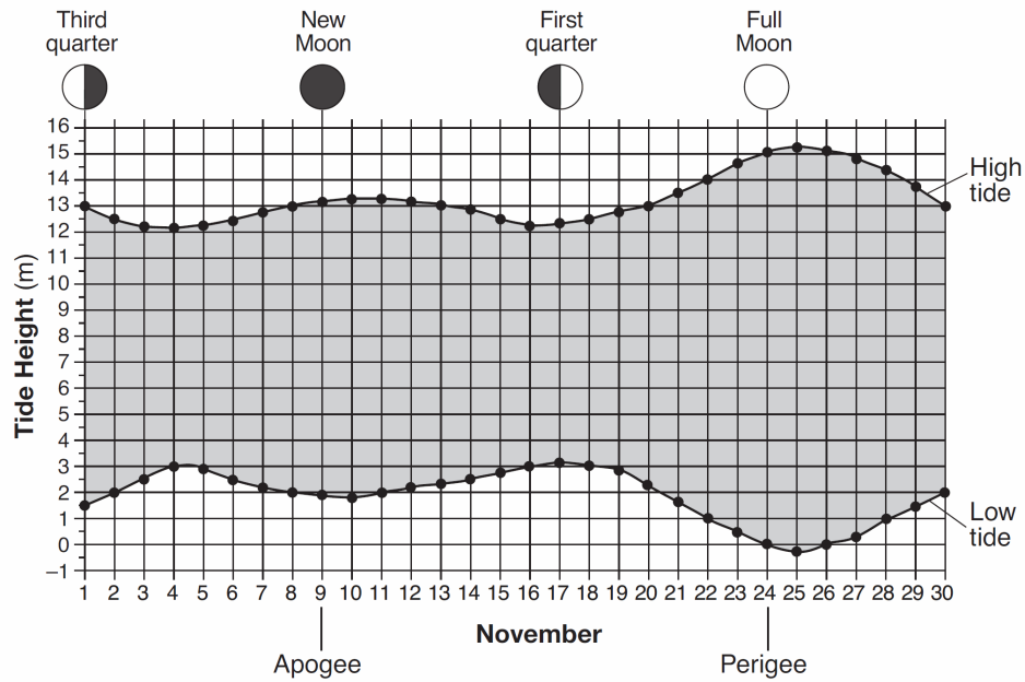
November 2007 Tidal Range – Minas Basin, Nova Scotia
